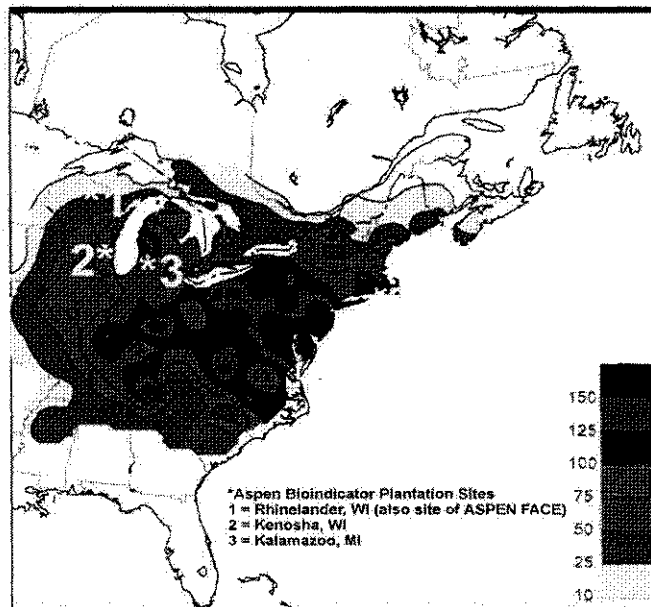
Fig. 1. Spatial distribution of average hours with ozone >82 ppb (1986-1993) (from: Dann and Summers, 1997) and locations of aspen plantations (1, 2, 3).
